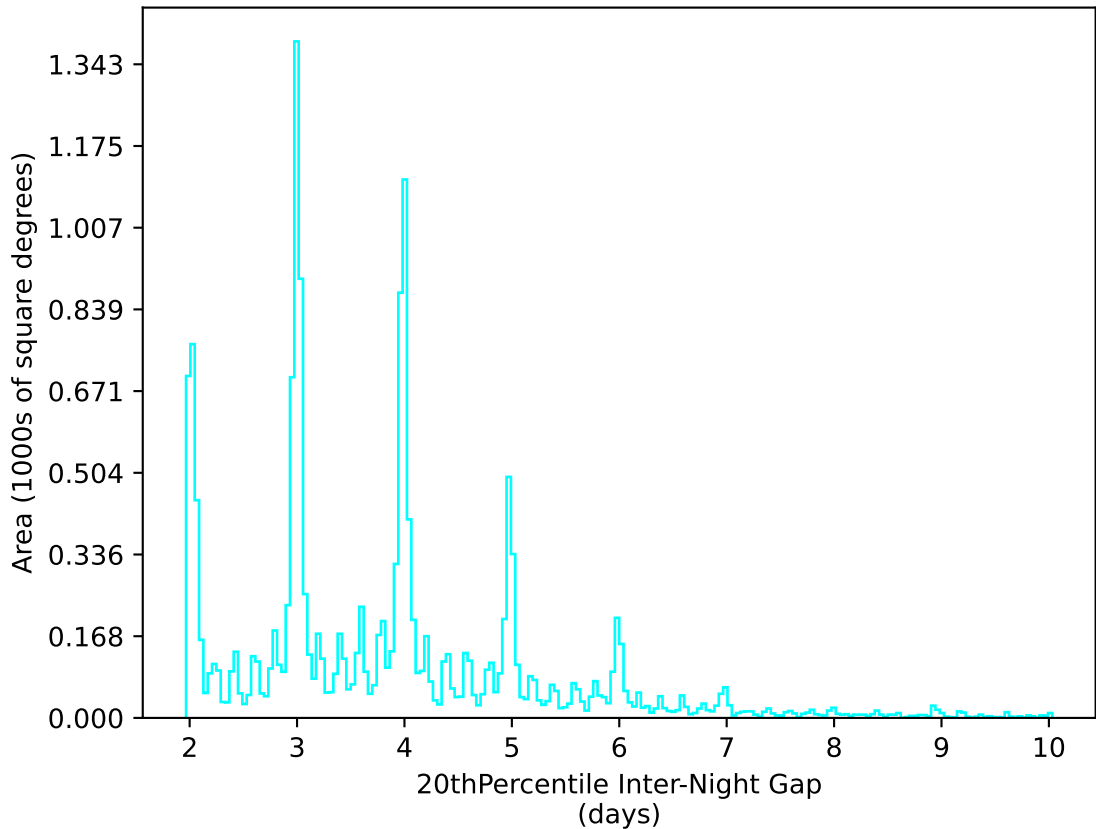
extra_ss_neo7_v3.4_10yrs WFD u band: 20thPercentile Inter-Night Gap
