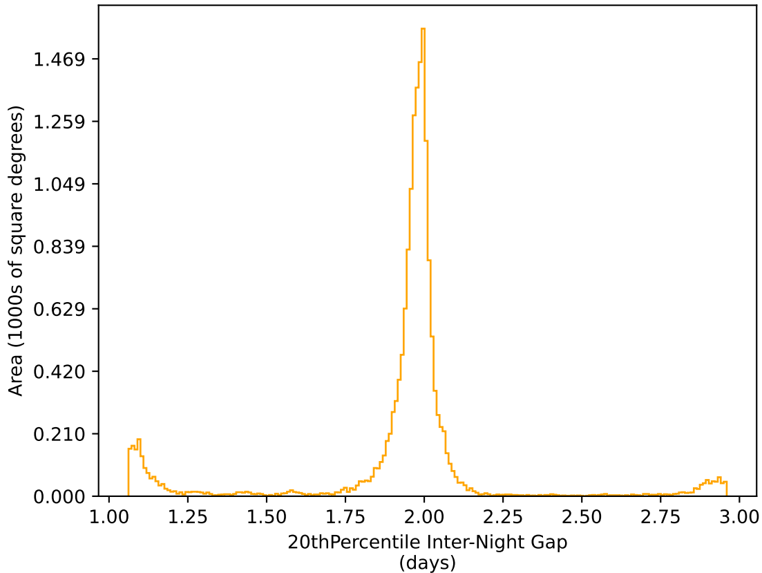
extra_ss_neo7_v3.4_10yrs WFD r band: 20thPercentile Inter-Night Gap
