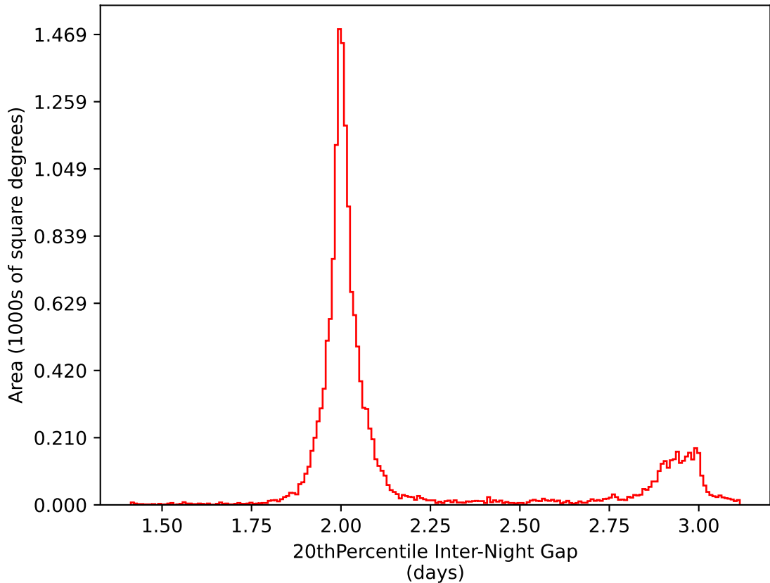
extra_ss_neo7_v3.4_10yrs WFD i band: 20thPercentile Inter-Night Gap
