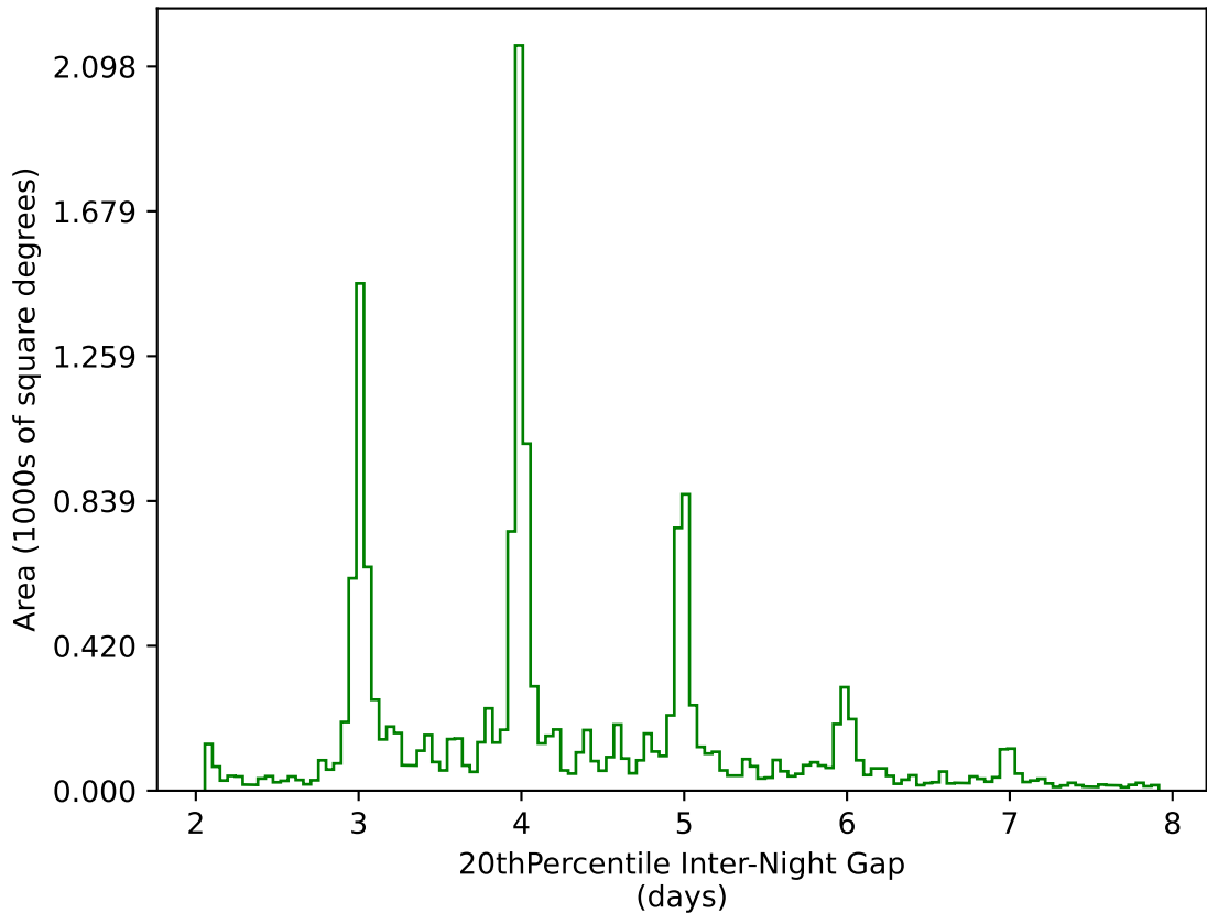
extra_ss_neo7_v3.4_10yrs WFD g band: 20thPercentile Inter-Night Gap
