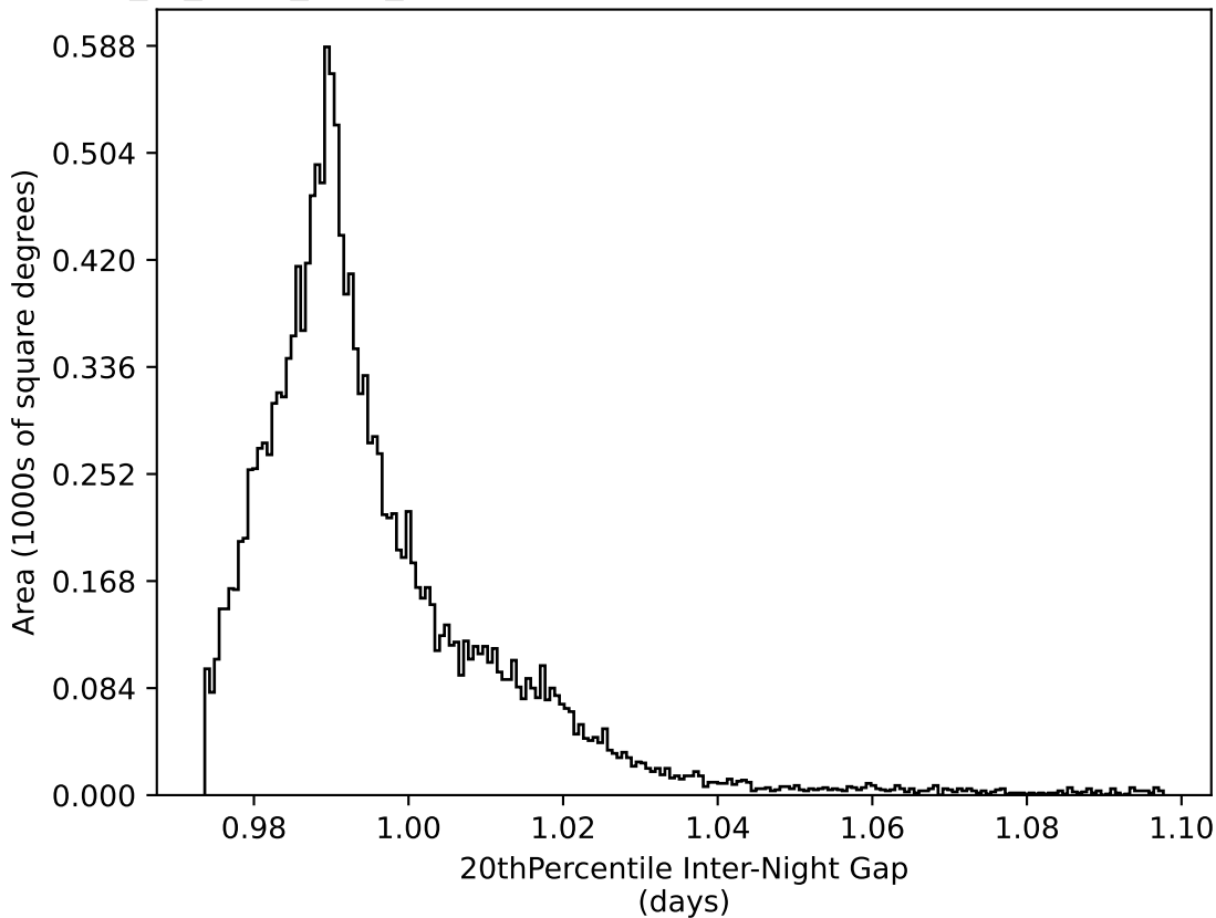
extra_ss_neo7_v3.4_10yrs WFD all bands: 20thPercentile Inter-Night Gap
