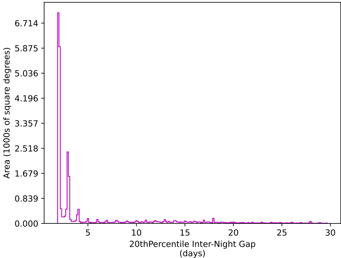
extra_ss_neo7_v3.4_10yrs All sky z band: 20thPercentile Inter-Night Gap
