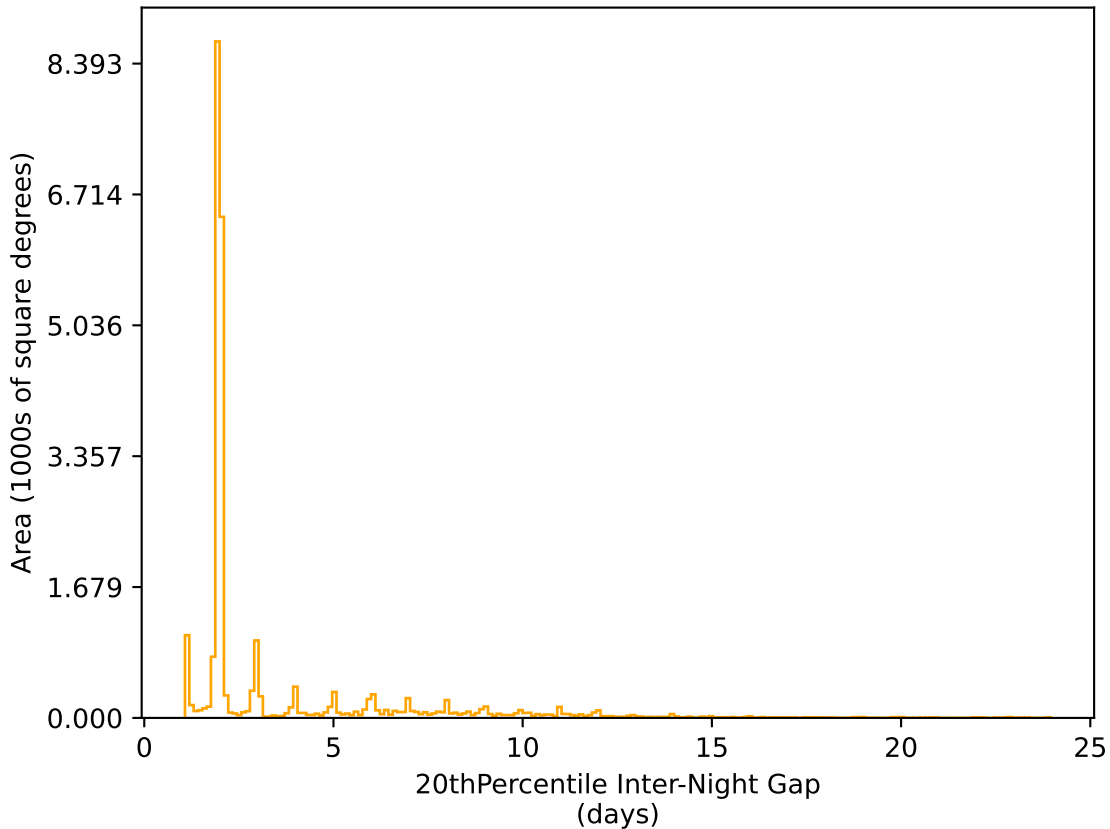
extra_ss_neo7_v3.4_10yrs All sky r band: 20thPercentile Inter-Night Gap
