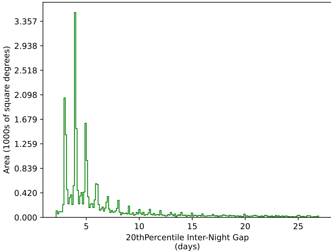
extra_ss_neo7_v3.4_10yrs All sky g band: 20thPercentile Inter-Night Gap
