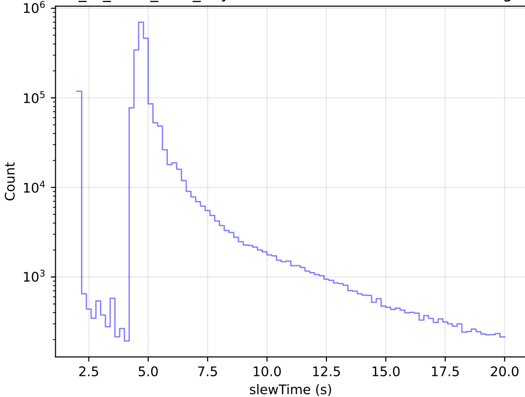
extra_ss_neo7_v3.4_10yrs All visits: Zoom Slew Time Histogram
