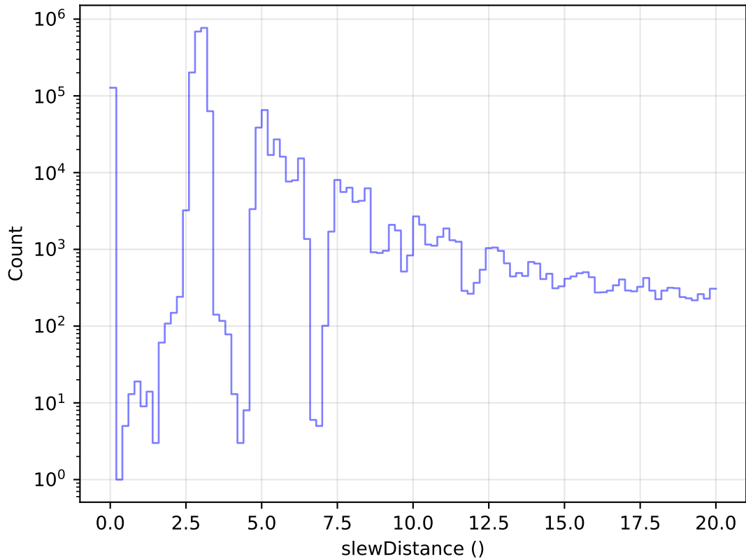
extra_ss_neo7_v3.4_10yrs All visits: Zoom Slew Distance Histogram
