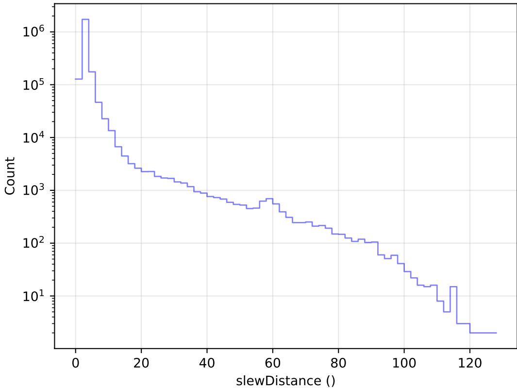
extra_ss_neo7_v3.4_10yrs All visits: Slew Distance Histogram
