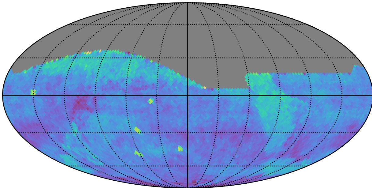
extra_ss_neo7_v3.4_10yrs (g or r or i): PairFraction
