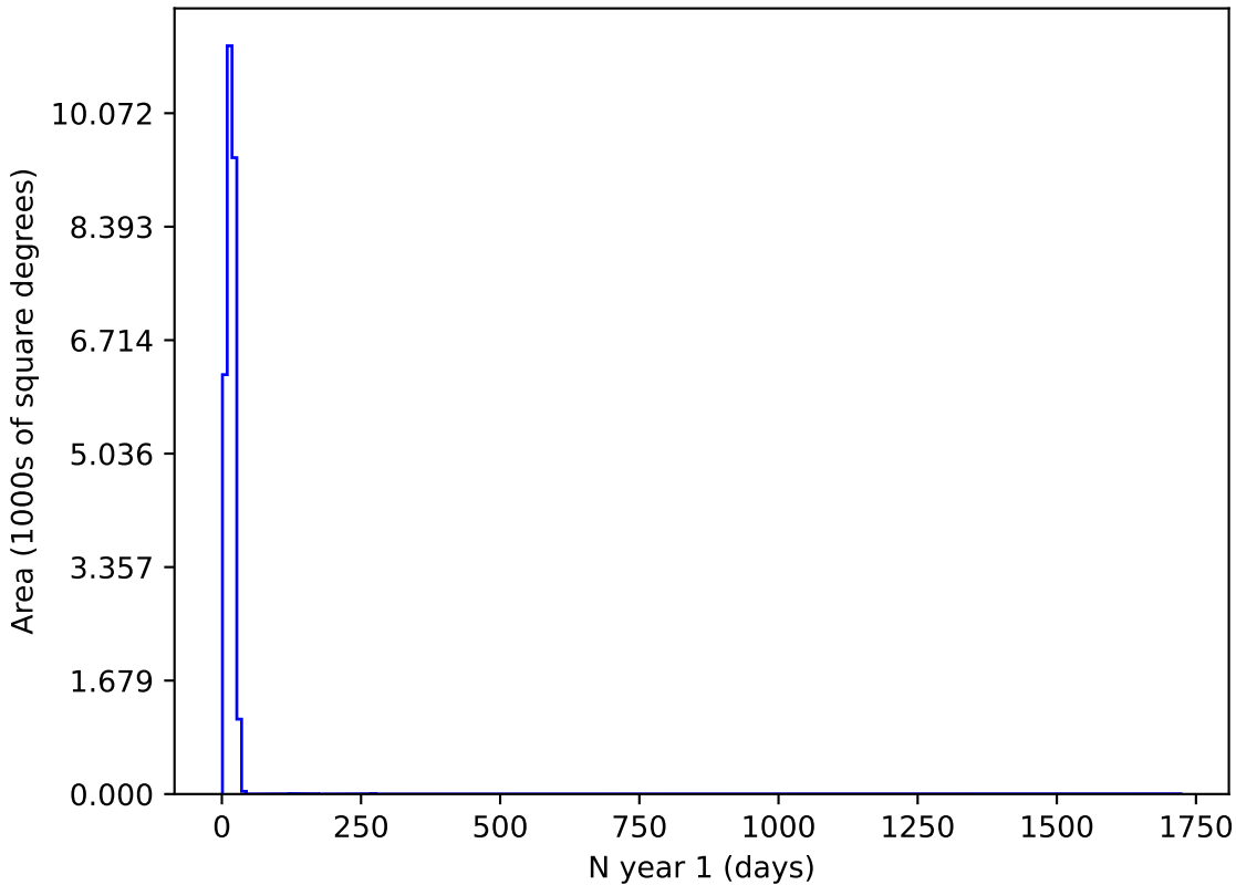
extra_ss_neo7_v3.4_10yrs r and night < 365: N year 1
