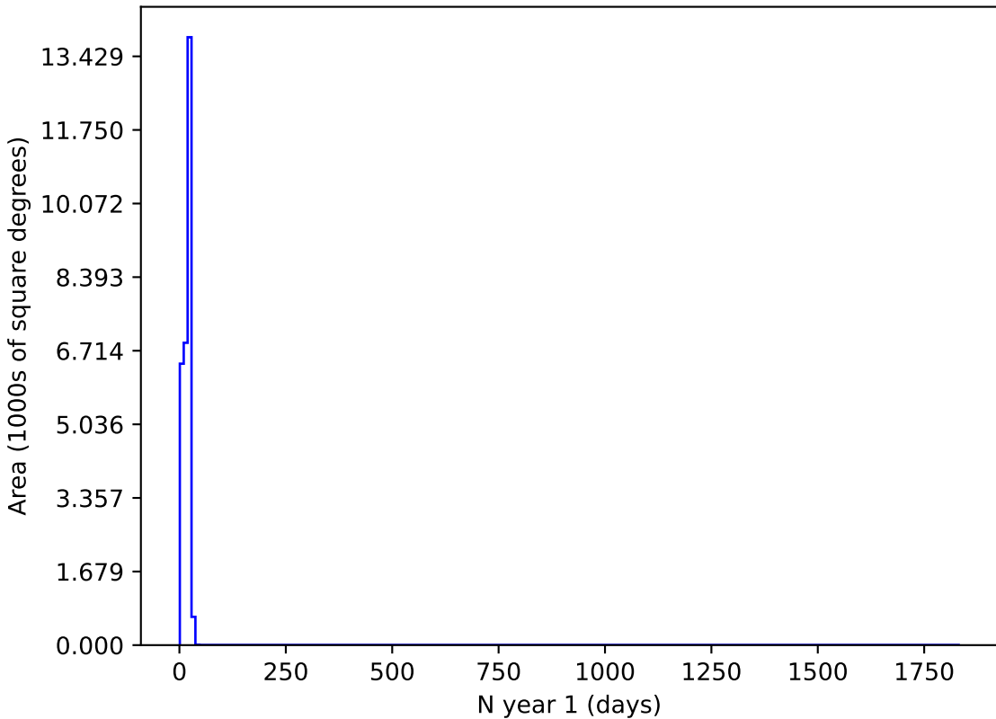
extra_ss_neo7_v3.4_10yrs i and night < 365: N year 1
