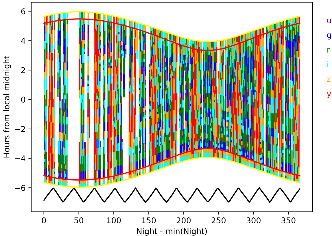
extra_ss_neo7_v3.4_10yrs year 8-9: Hourglass
