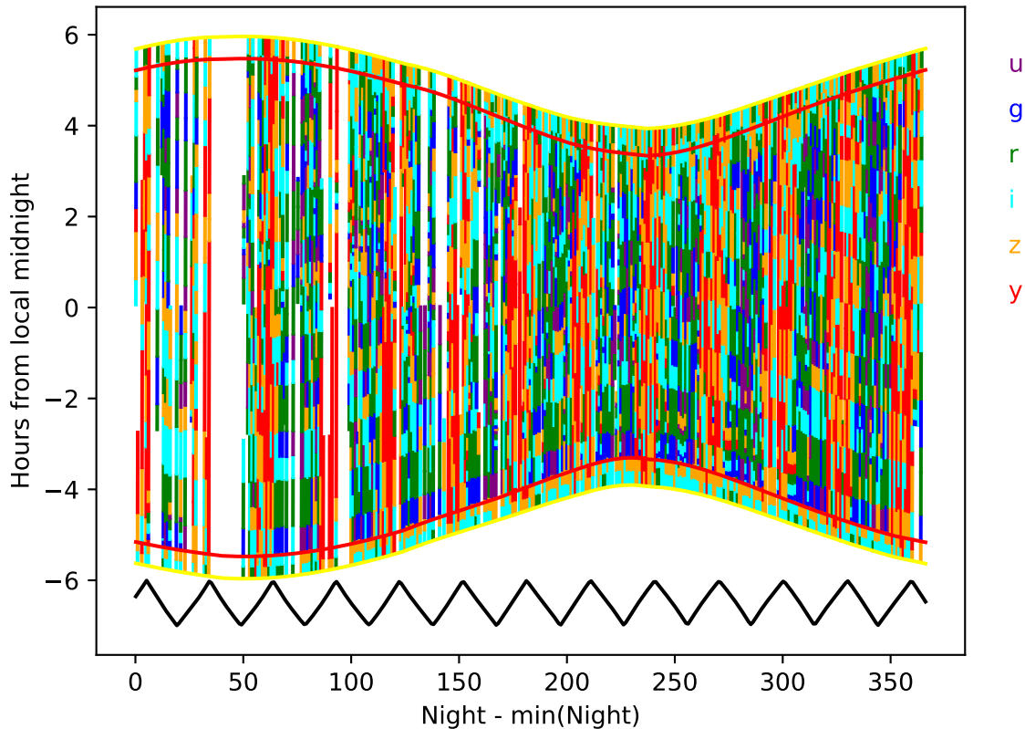
extra_ss_neo7_v3.4_10yrs year 6-7: Hourglass
