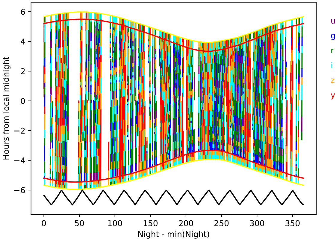
extra_ss_neo7_v3.4_10yrs year 4-5: Hourglass
