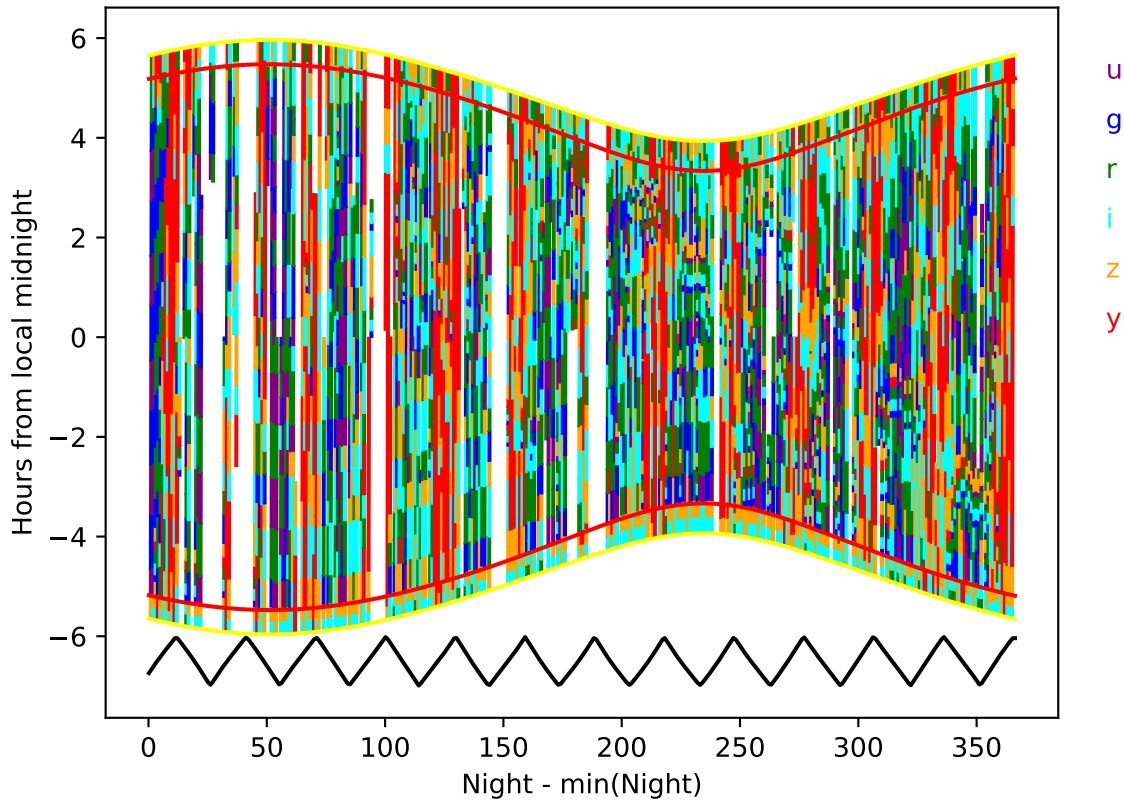
extra_ss_neo7_v3.4_10yrs year 0-1: Hourglass
