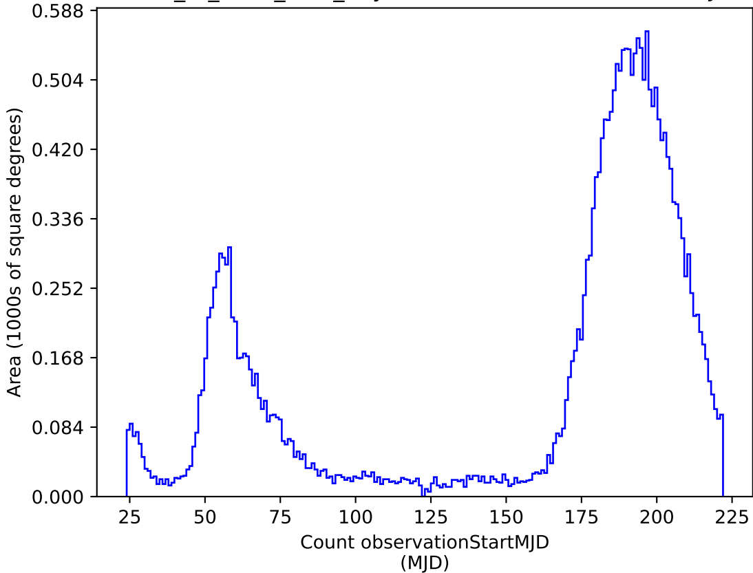
extra_ss_neo7_v3.4_10yrs i: Count observationStartMJD
