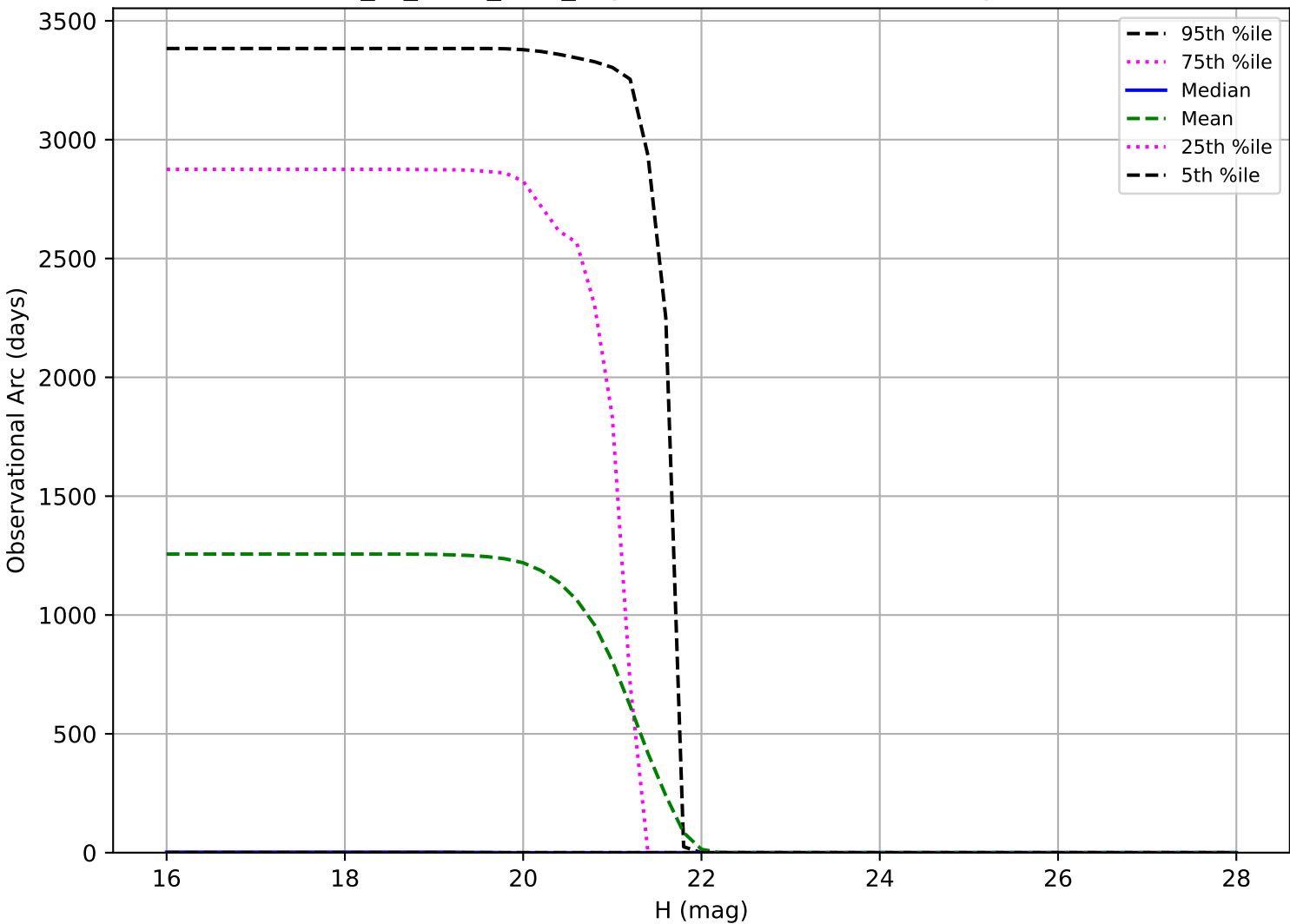
extra_ss_neo5_v3.4_10yrs: Observational Arc Length Vatira
