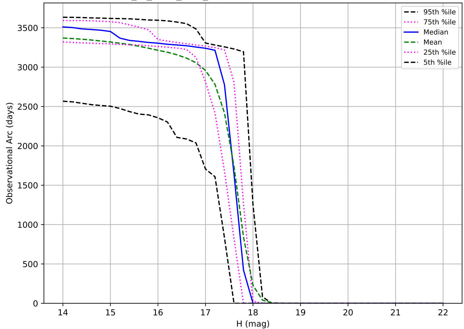
extra_ss_neo5_v3.4_10yrs: Observational Arc Length Trojan
