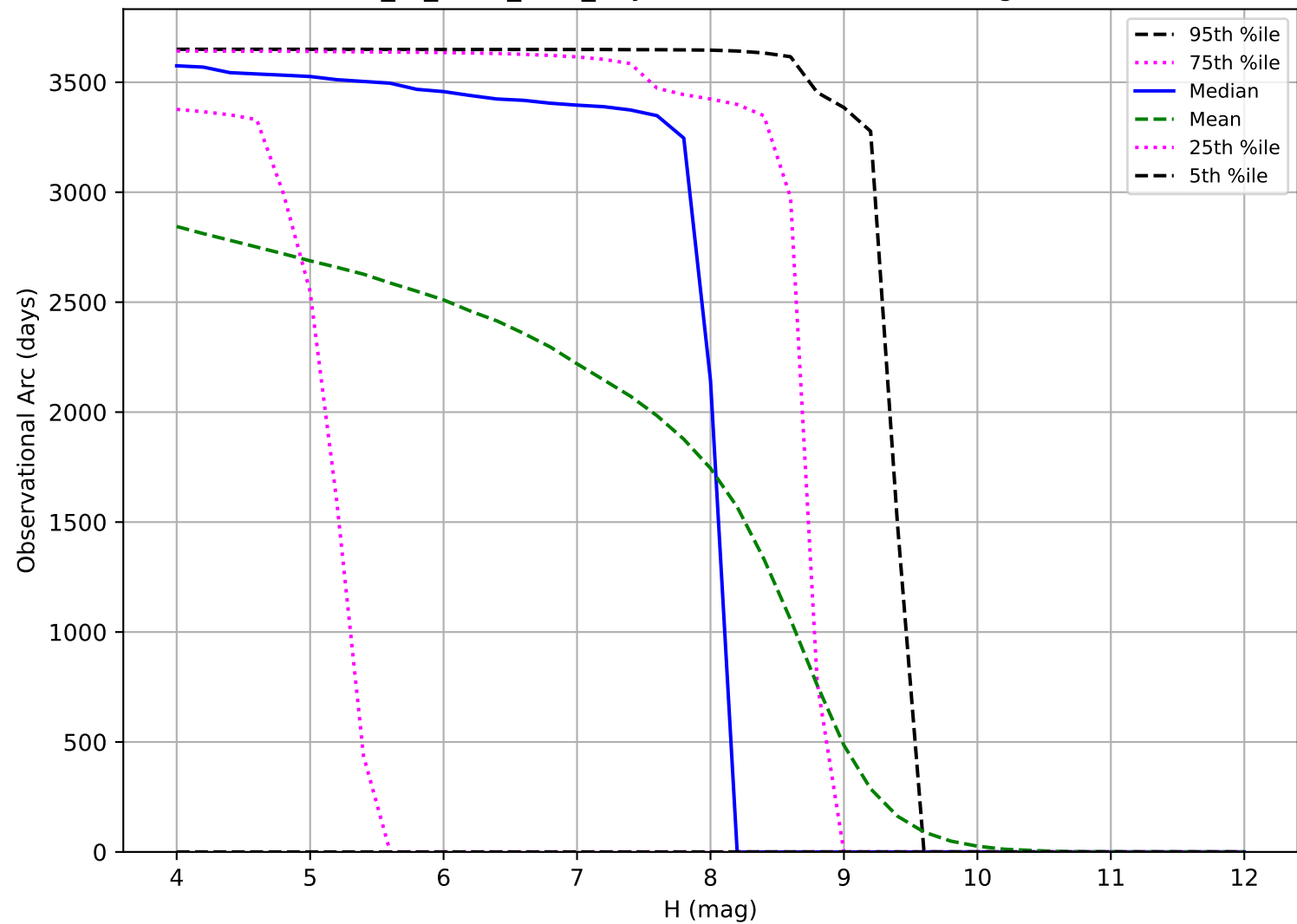
extra_ss_neo5_v3.4_10yrs: Observational Arc Length TNO
