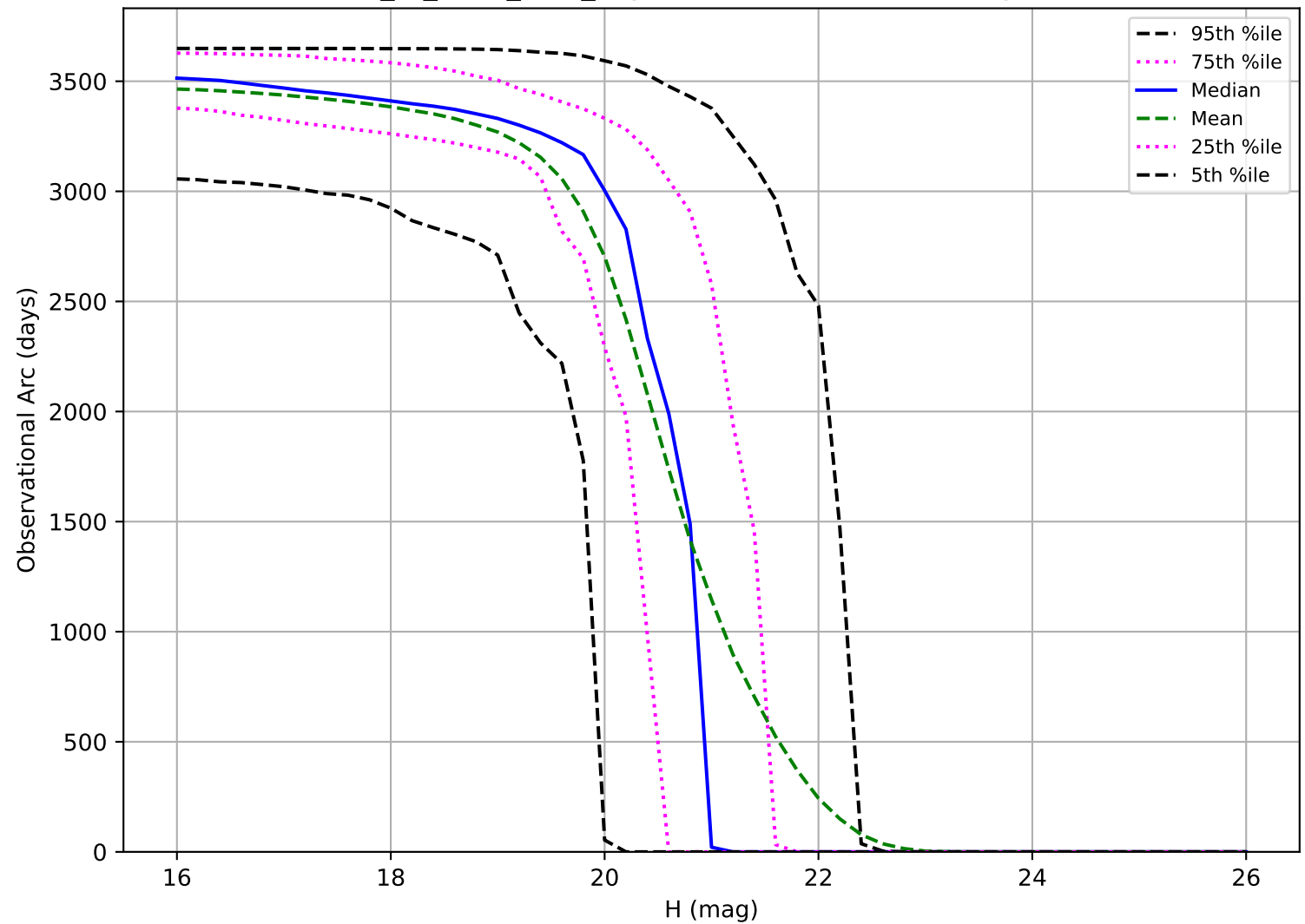
extra_ss_neo5_v3.4_10yrs: Observational Arc Length MBA
