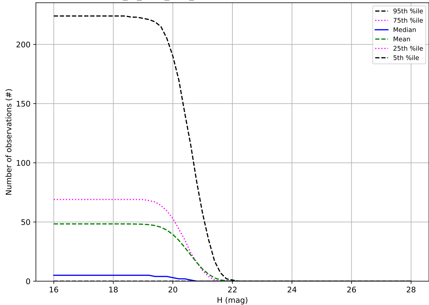
extra_ss_neo5_v3.4_10yrs: Number of observations Vatira
