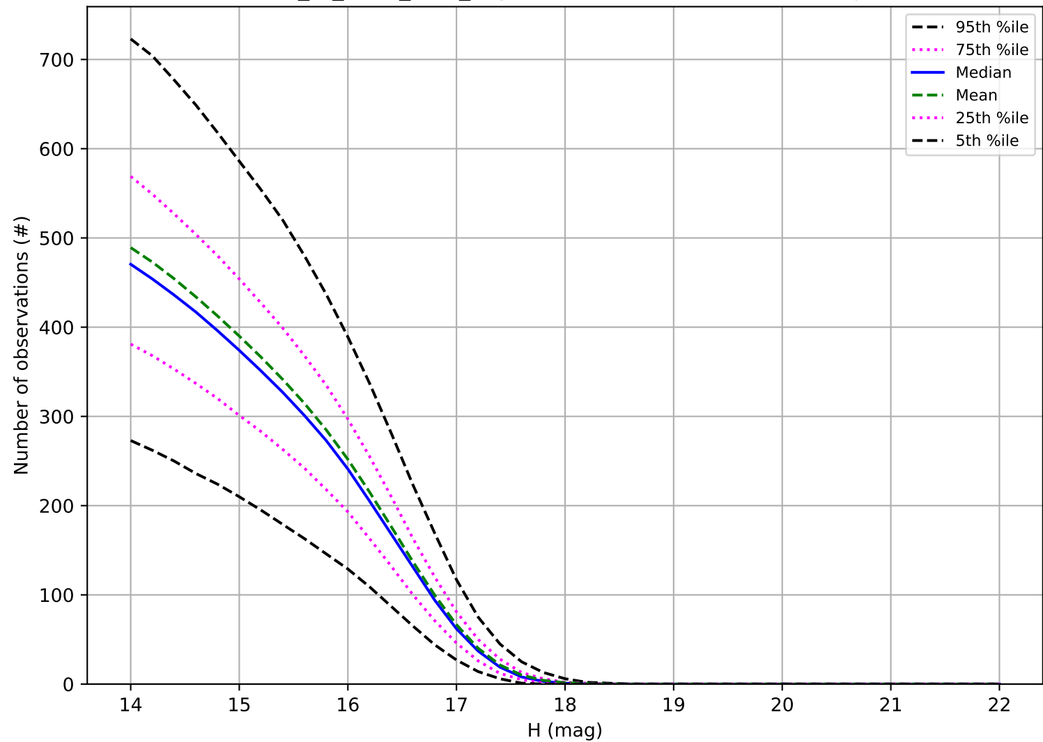
extra_ss_neo5_v3.4_10yrs: Number of observations Trojan
