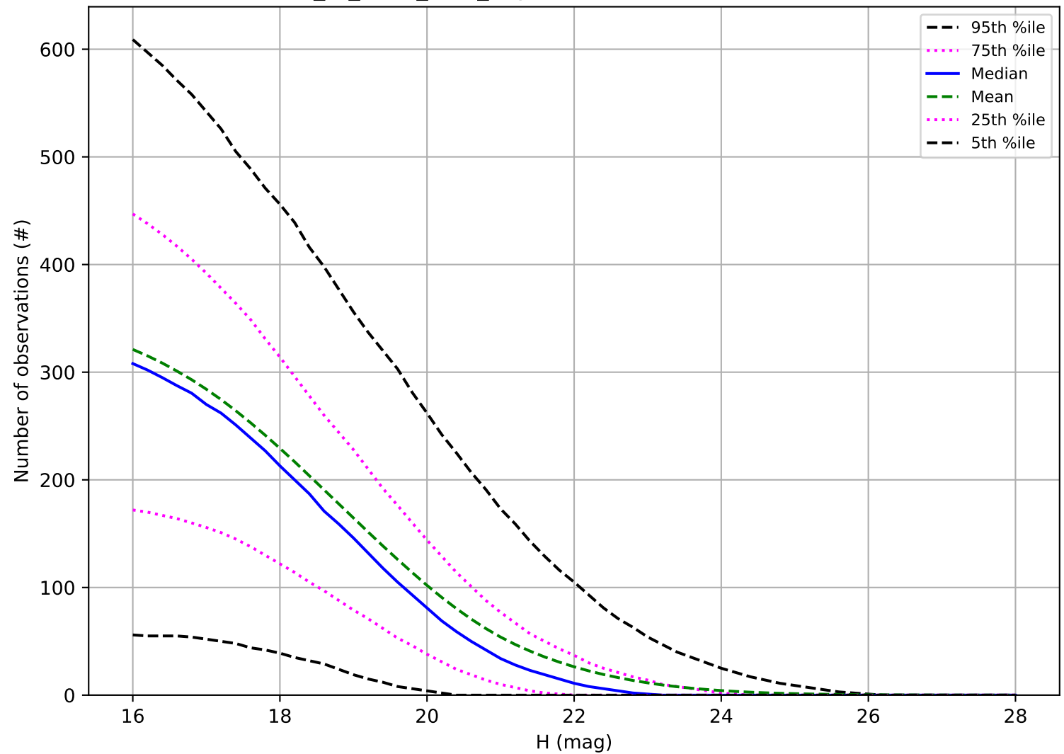
extra_ss_neo5_v3.4_10yrs: Number of observations PHA
