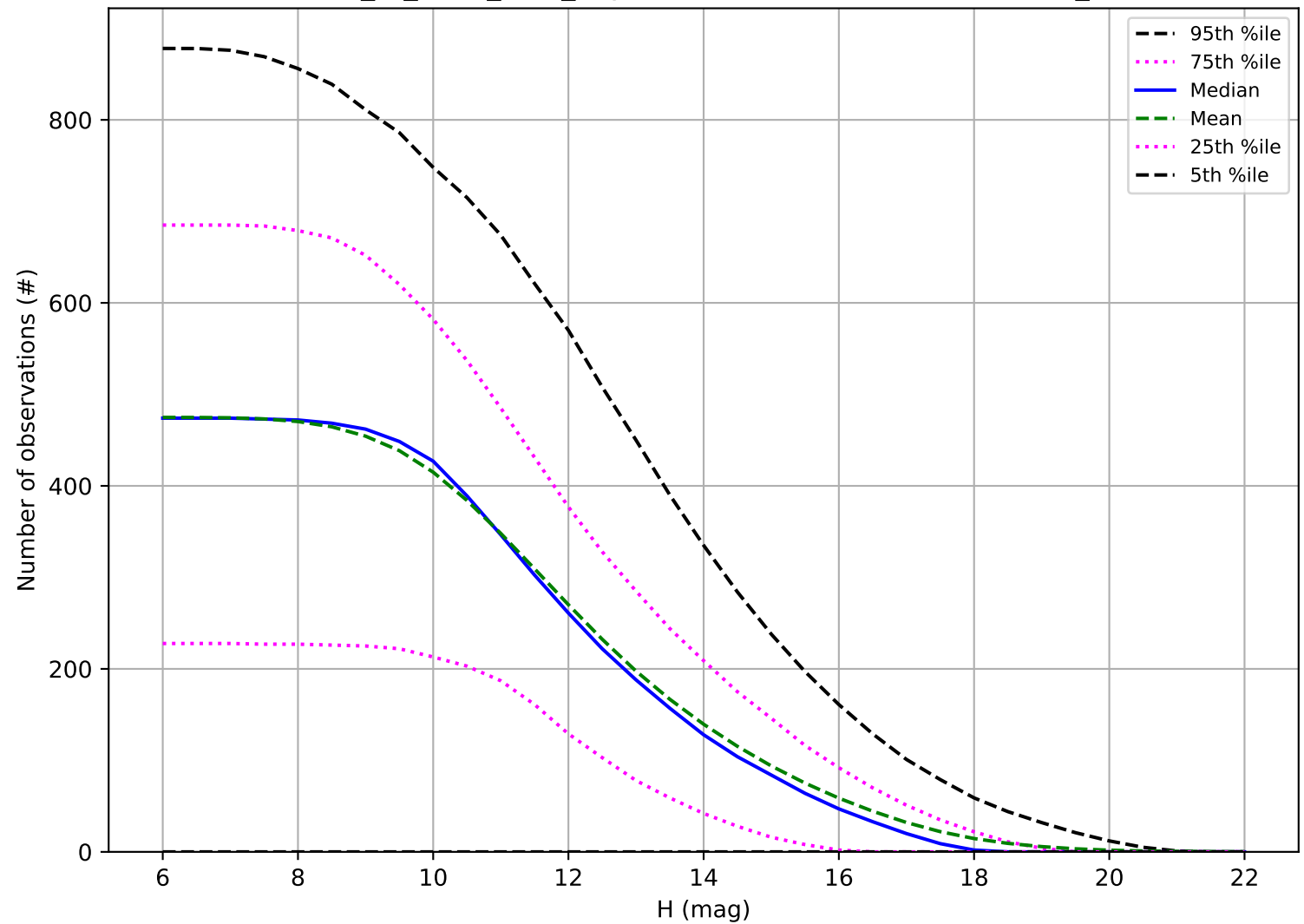
extra_ss_neo5_v3.4_10yrs: Number of observations OCC_r5
