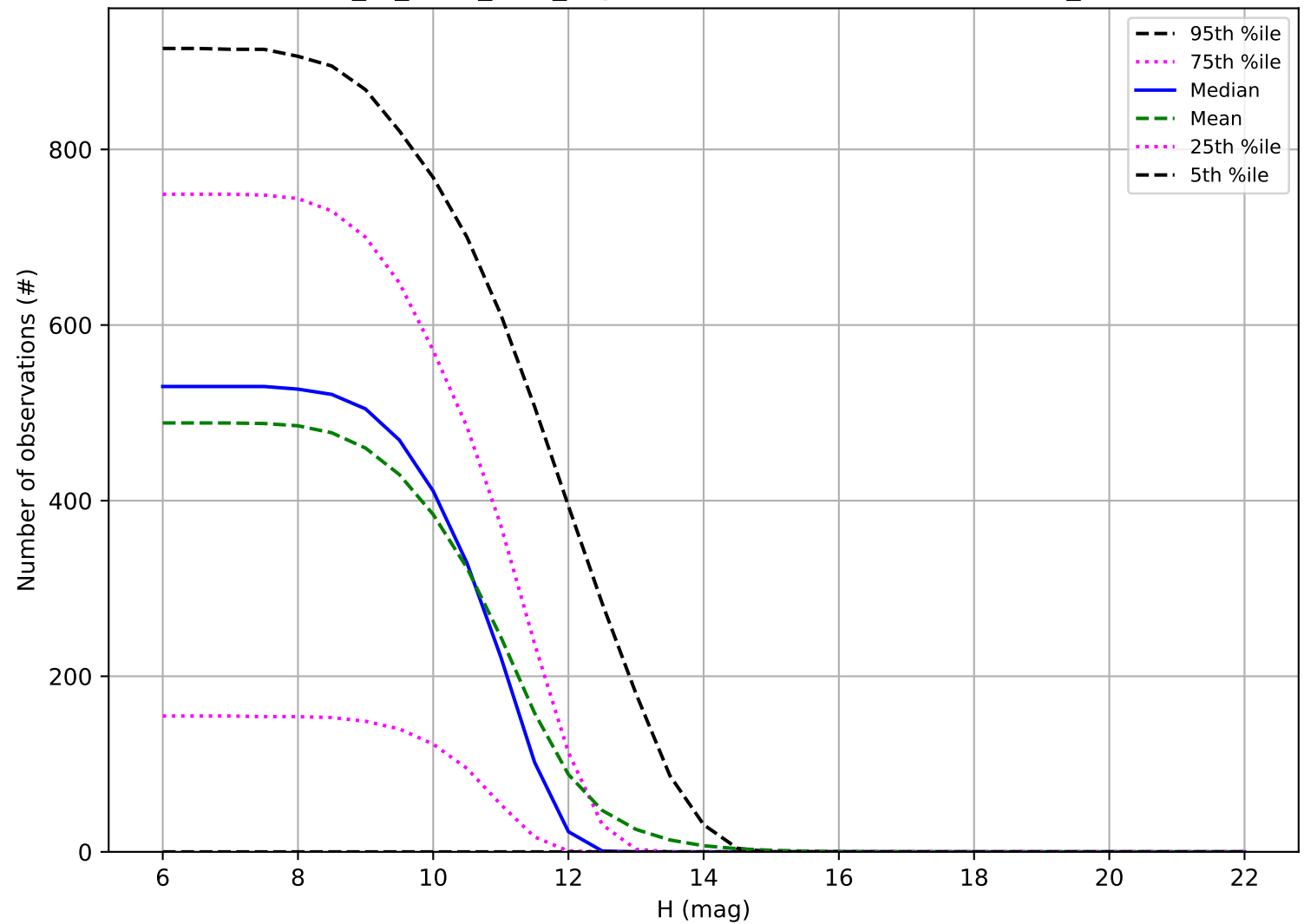
extra_ss_neo5_v3.4_10yrs: Number of observations OCC_r20
