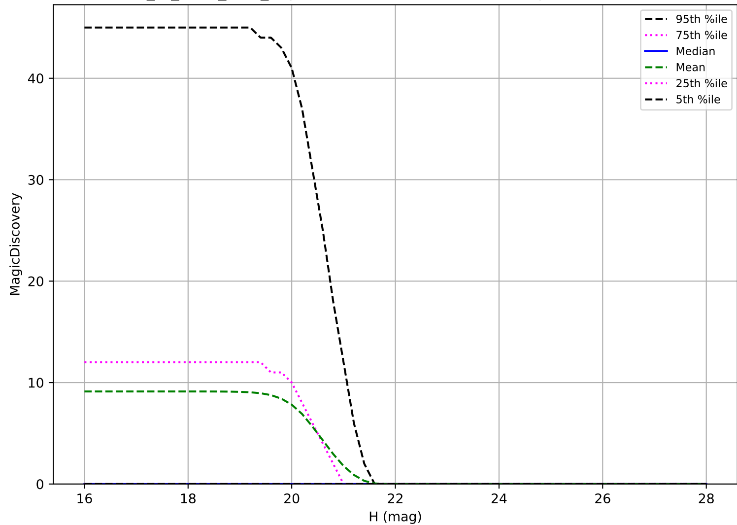
extra_ss_neo5_v3.4_10yrs: Vatira 6 detections in 60 nights detection loss
