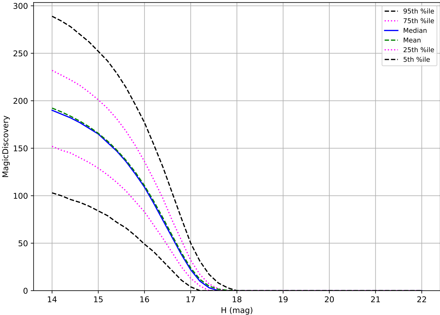
extra_ss_neo5_v3.4_10yrs: Trojan 6 detections in 60 nights detection loss
