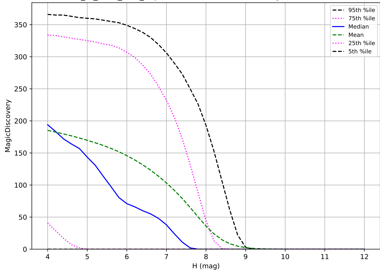
extra_ss_neo5_v3.4_10yrs: TNO 6 detections in 60 nights detection loss
