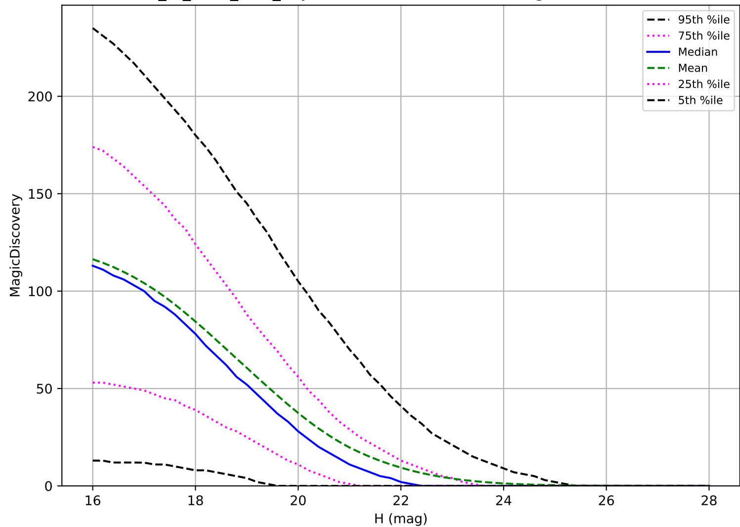
extra_ss_neo5_v3.4_10yrs: PHA 6 detections in 60 nights detection loss
