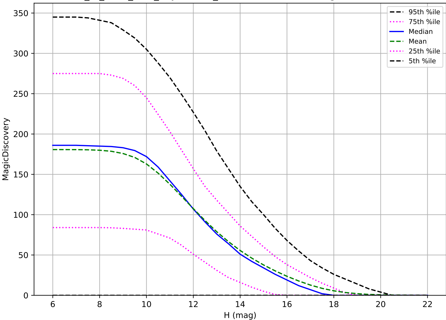
extra_ss_neo5_v3.4_10yrs: OCC_r5 6 detections in 60 nights detection loss
