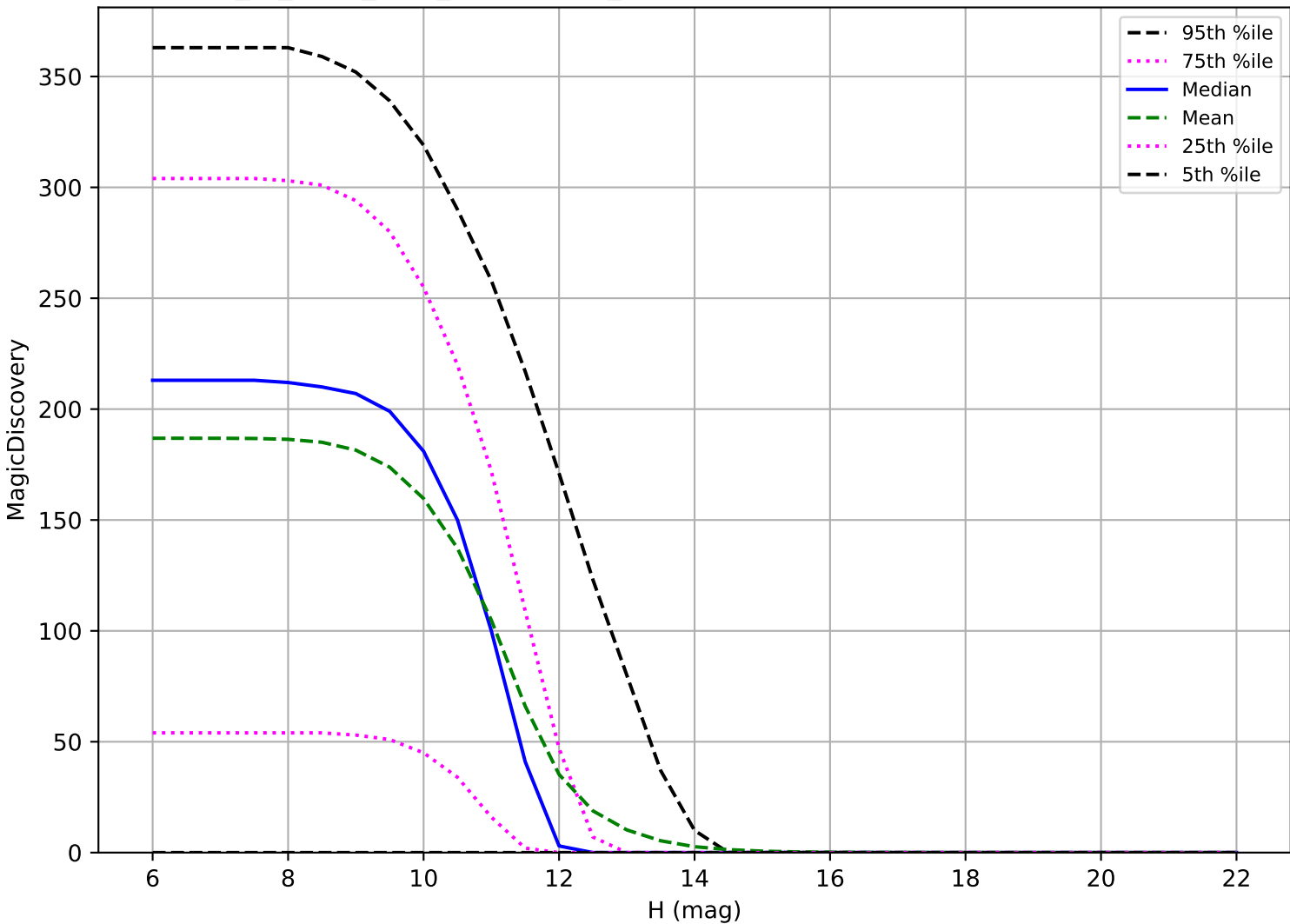
extra_ss_neo5_v3.4_10yrs: OCC_r20 6 detections in 60 nights detection loss
