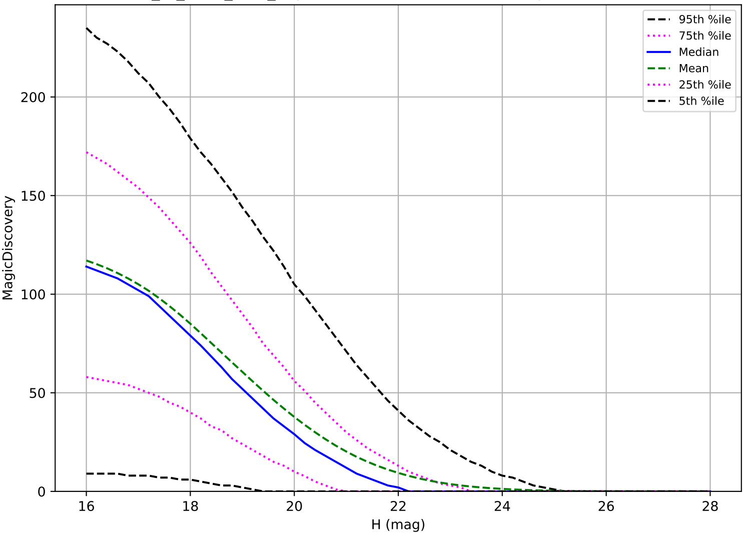
extra_ss_neo5_v3.4_10yrs: NEO 6 detections in 60 nights detection loss
