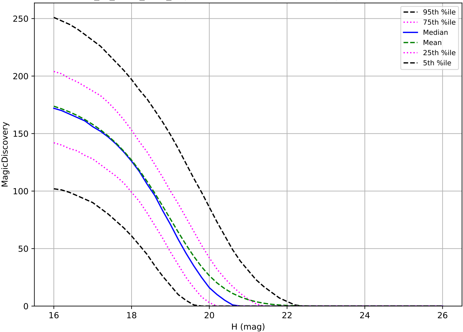
extra_ss_neo5_v3.4_10yrs: MBA 6 detections in 60 nights detection loss
