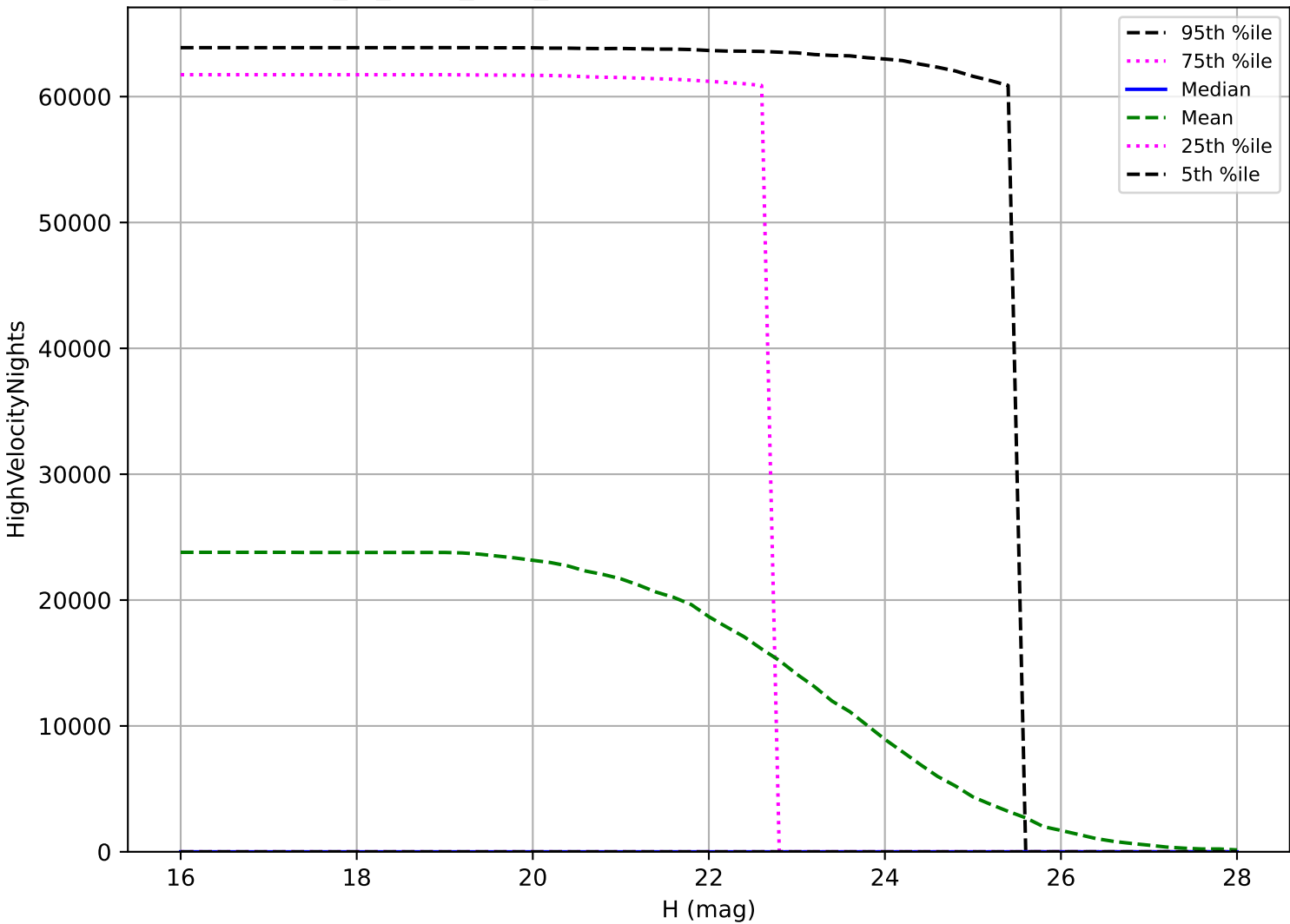
extra_ss_neo5_v3.4_10yrs: PHA High velocity pair detection loss
