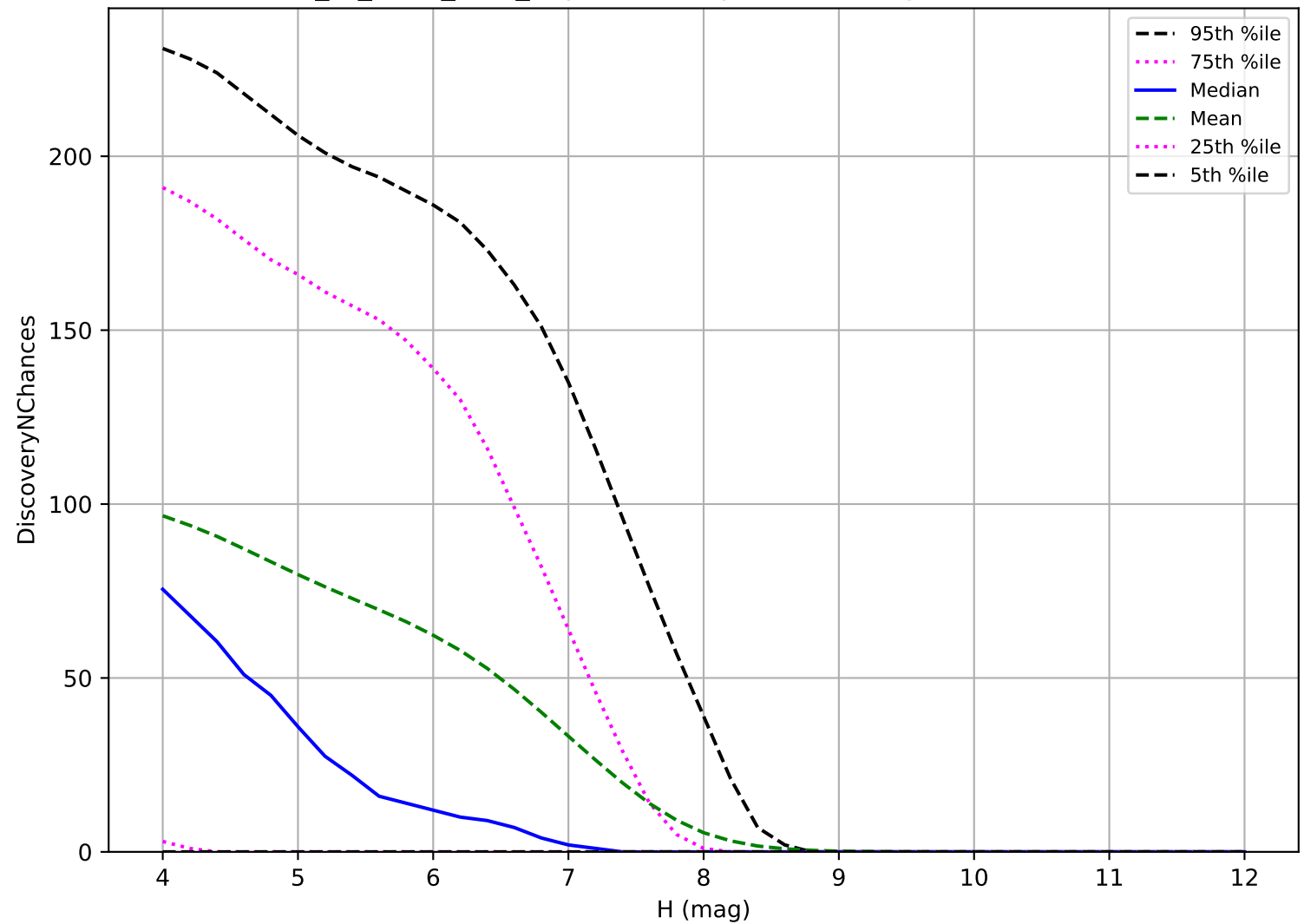
extra_ss_neo5_v3.4_10yrs: TNO 3 pairs in 15 nights detection loss
