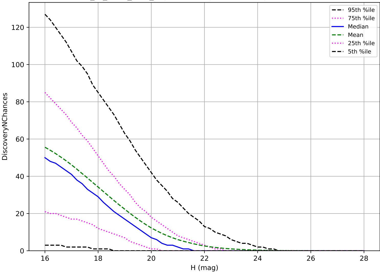
extra_ss_neo5_v3.4_10yrs: PHA 3 pairs in 15 nights detection loss
