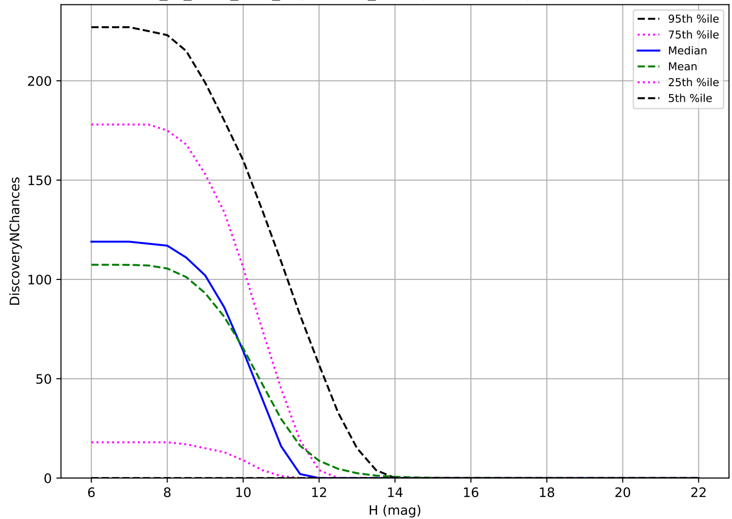
extra_ss_neo5_v3.4_10yrs: OCC_r20 3 pairs in 15 nights detection loss
