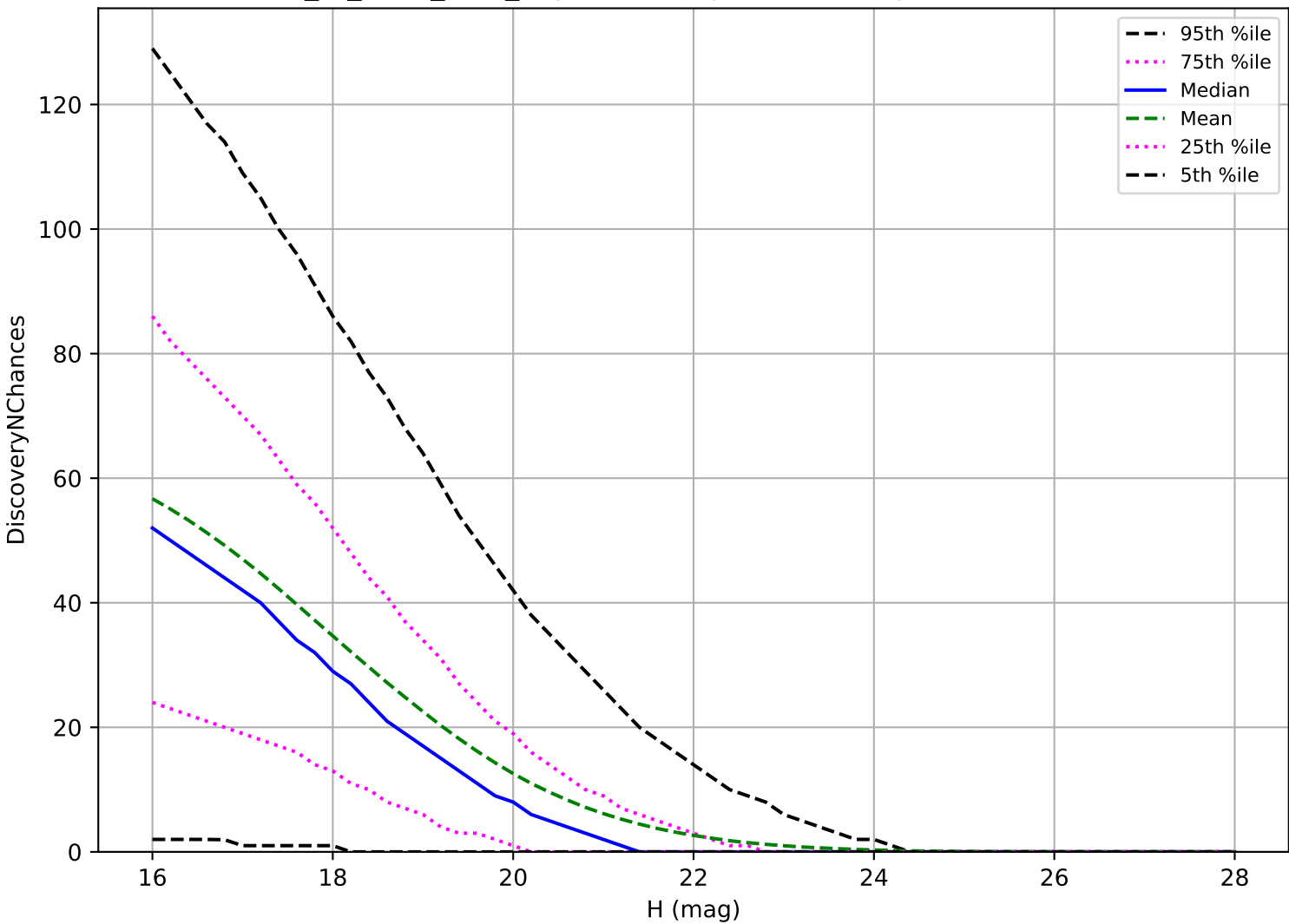
extra_ss_neo5_v3.4_10yrs: NEO 3 pairs in 15 nights detection loss
