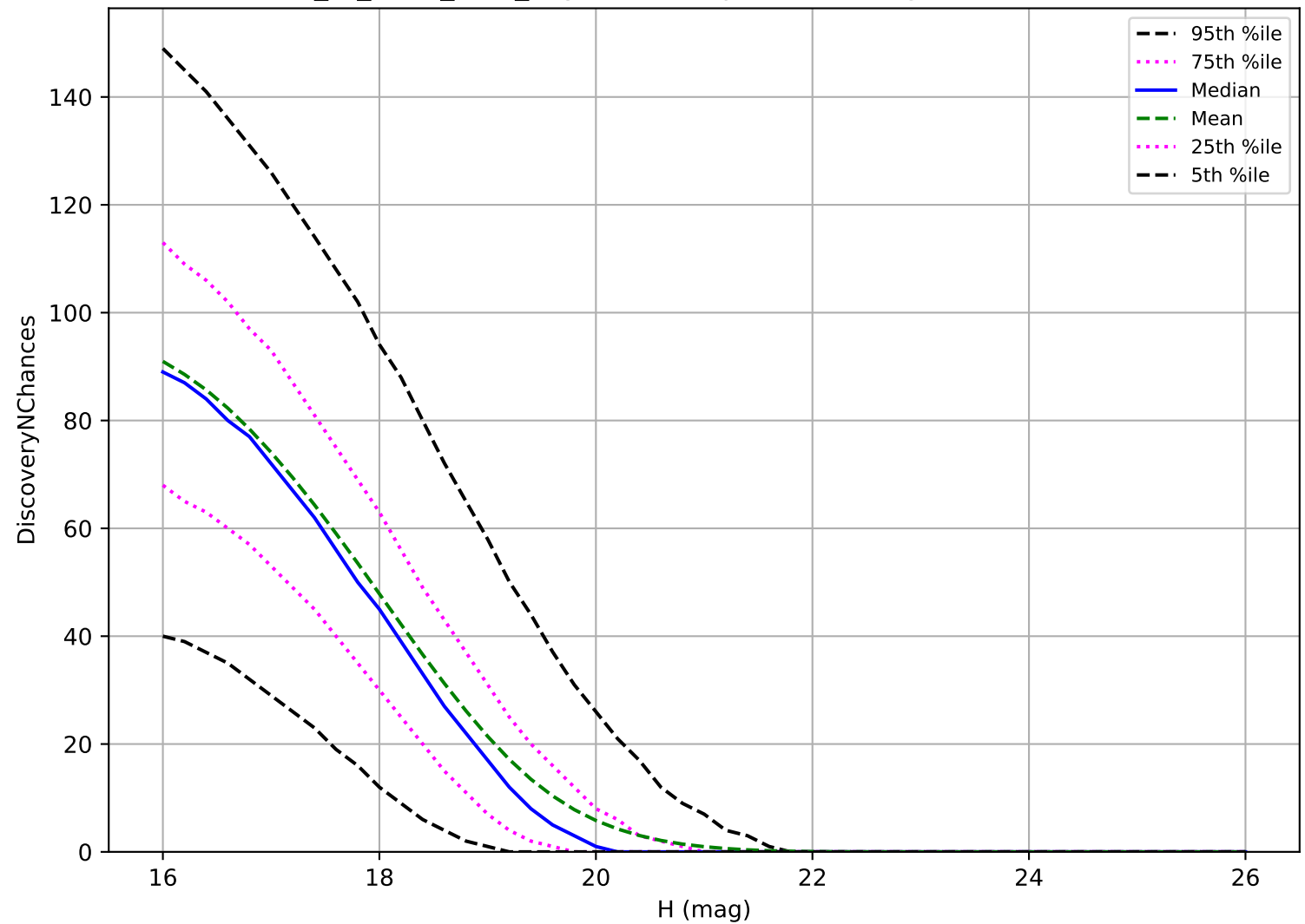
extra_ss_neo5_v3.4_10yrs: MBA 3 pairs in 15 nights detection loss
