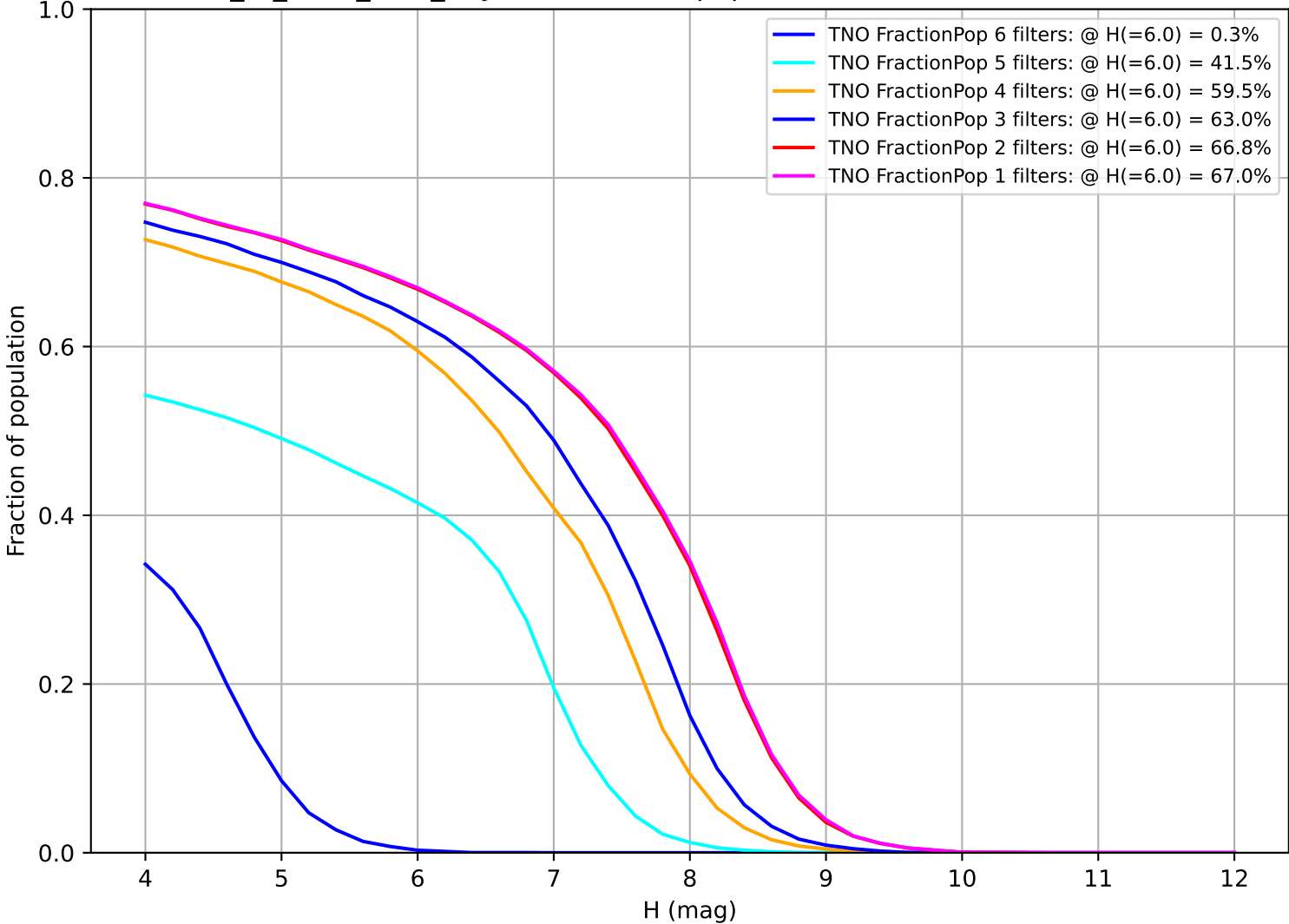
extra_ss_neo5_v3.4_10yrs: Fraction of population with colors in X filters TNO
