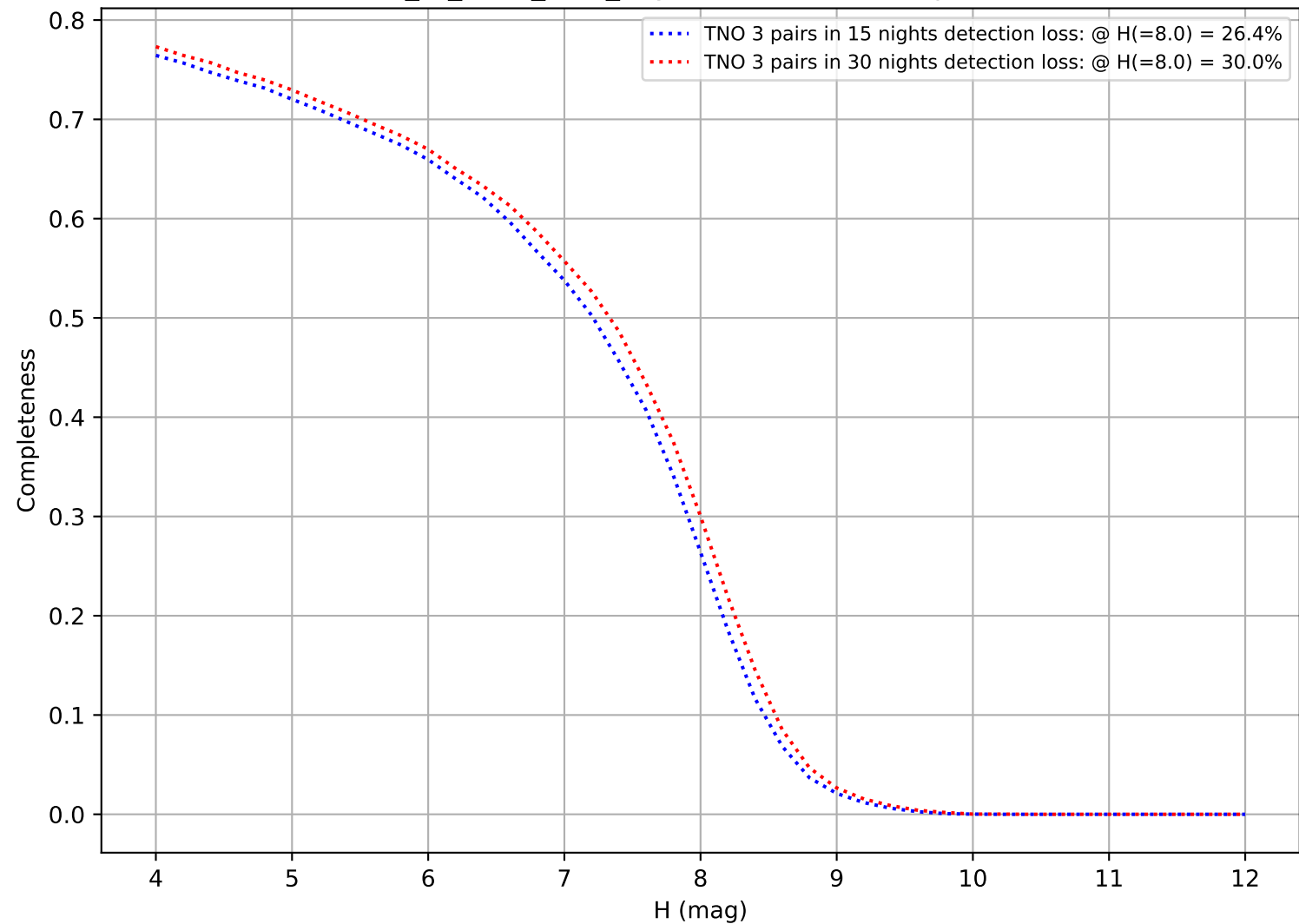
extra_ss_neo5_v3.4_10yrs: DifferentialCompleteness
