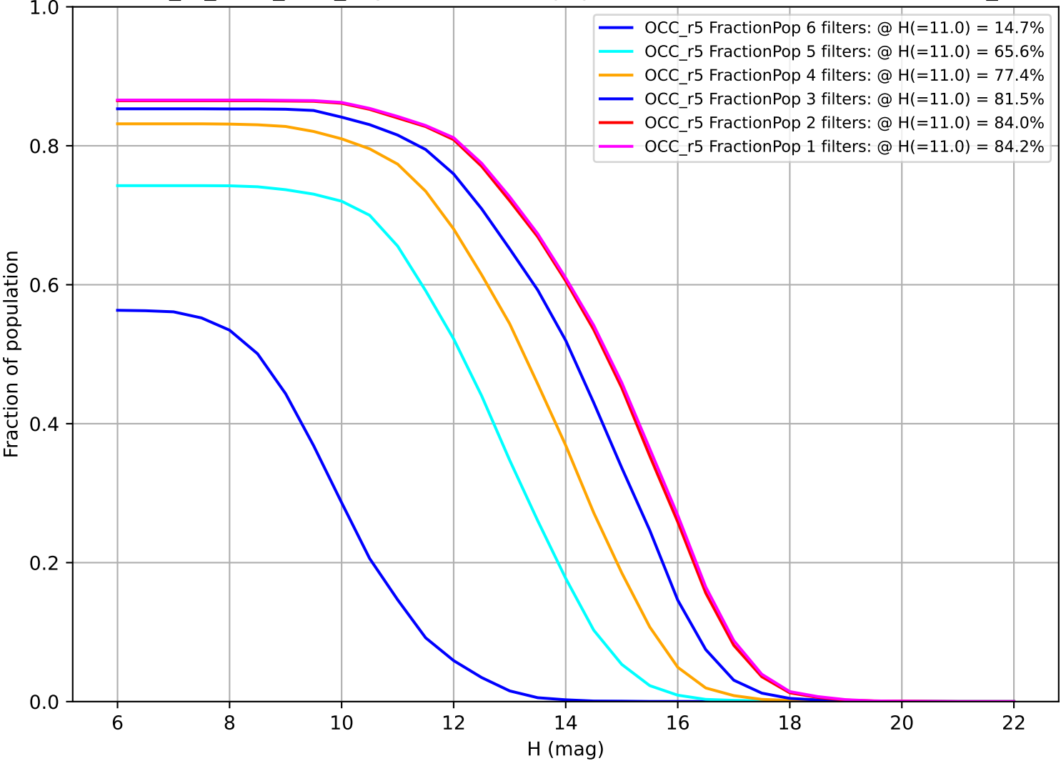
extra_ss_neo5_v3.4_10yrs: Fraction of population with colors in X filters OCC_r5
