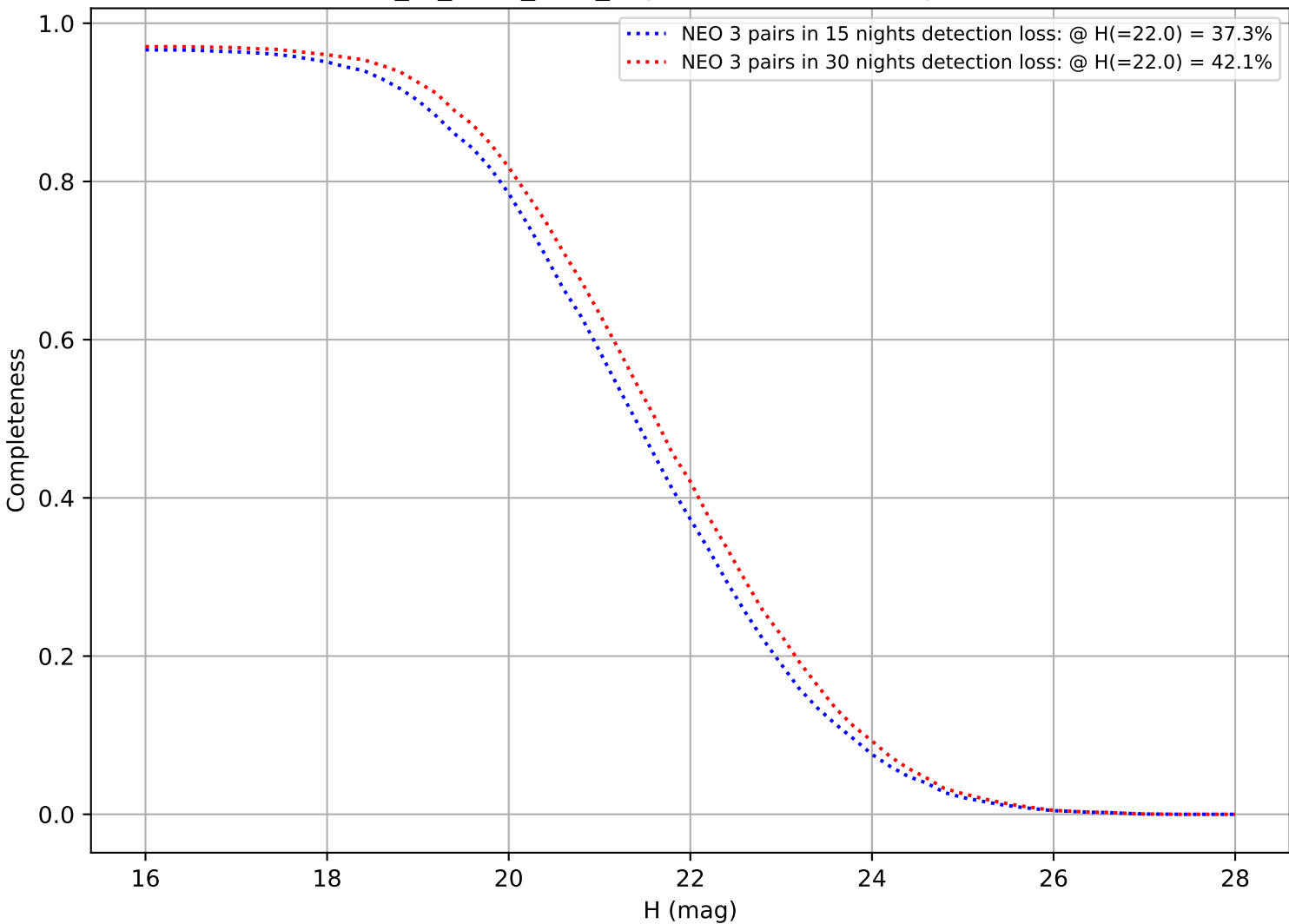
extra_ss_neo5_v3.4_10yrs: DifferentialCompleteness
