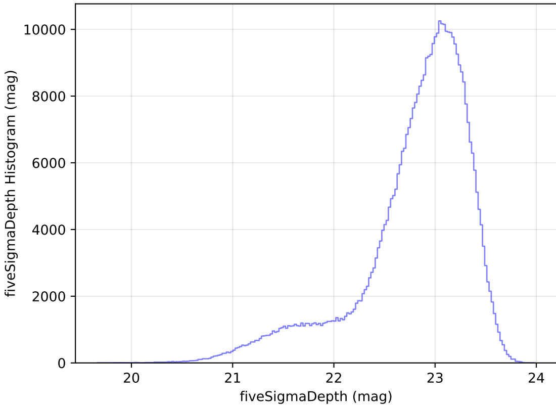
extra_ss_neo5_v3.4_10yrs z: fiveSigmaDepth Histogram
