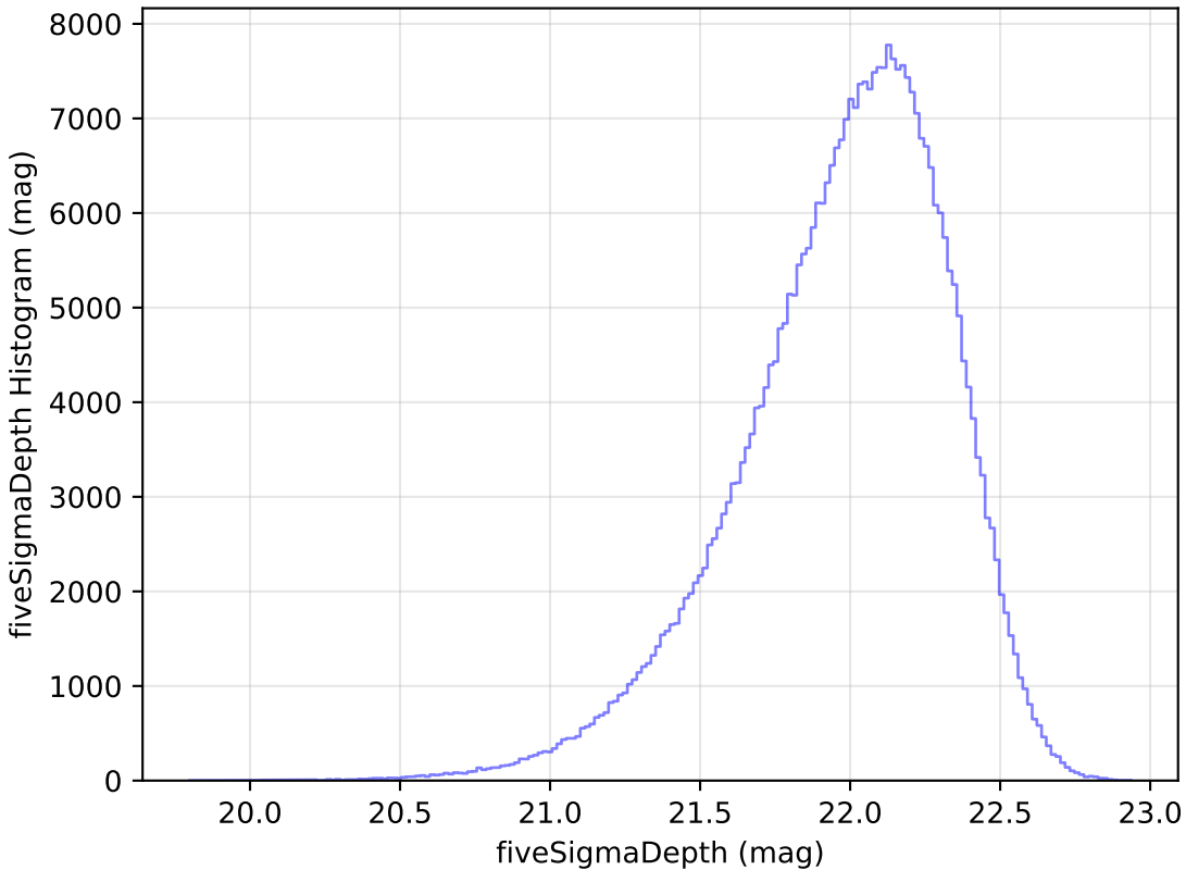
extra_ss_neo5_v3.4_10yrs y: fiveSigmaDepth Histogram
