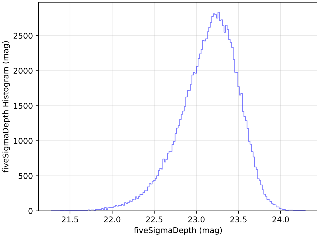
extra_ss_neo5_v3.4_10yrs u: fiveSigmaDepth Histogram
