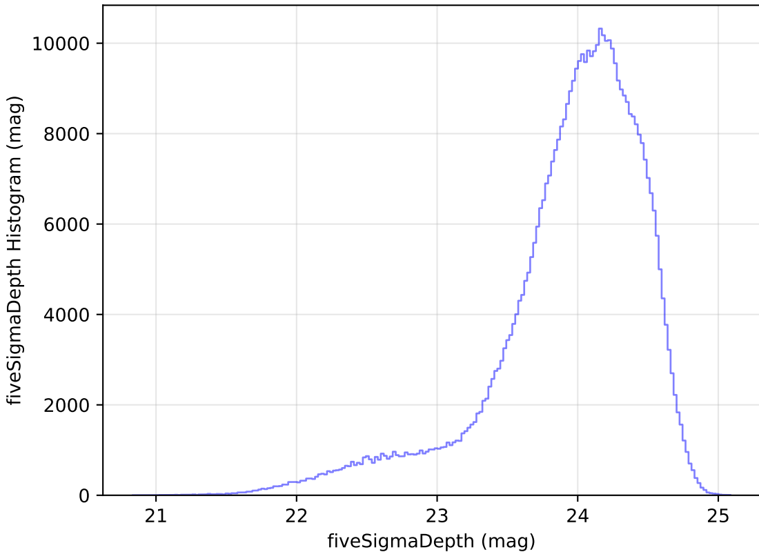
extra_ss_neo5_v3.4_10yrs r: fiveSigmaDepth Histogram
